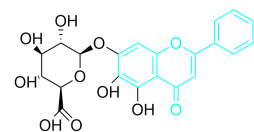
Baicalin
