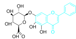
Baicalin
