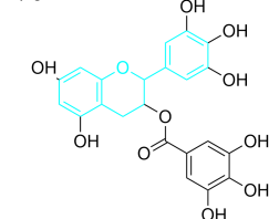
Epigallocatechin Gallate
