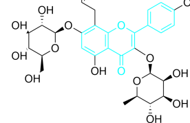
Icaritin
