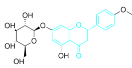
Biochanin A
