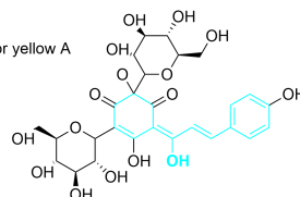
Quercetin
