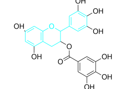
Epigallocatechin Gallate
